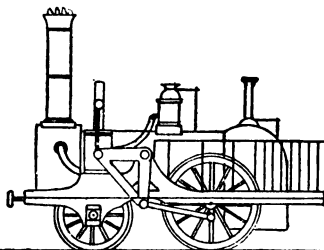
Fig. 31.—"Experiment," No. 32, Liverpool and Manchester Railway, 1833.
